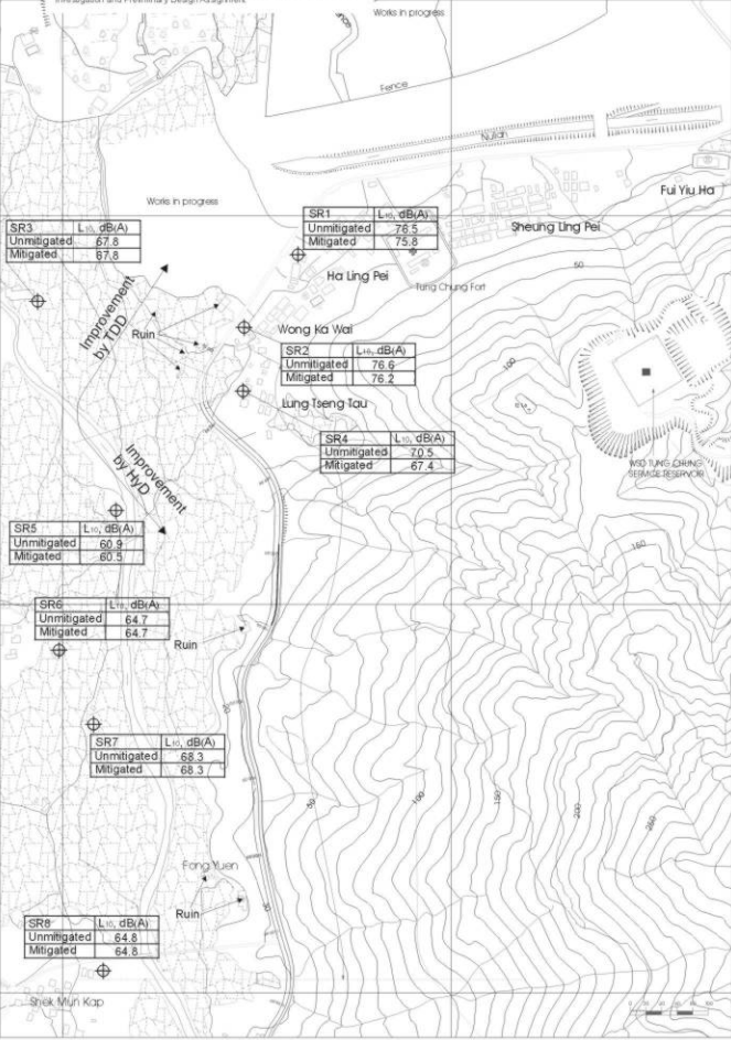
Maximum Unmitigated and Mitigated Operational Noise Levels at Representative NSR
